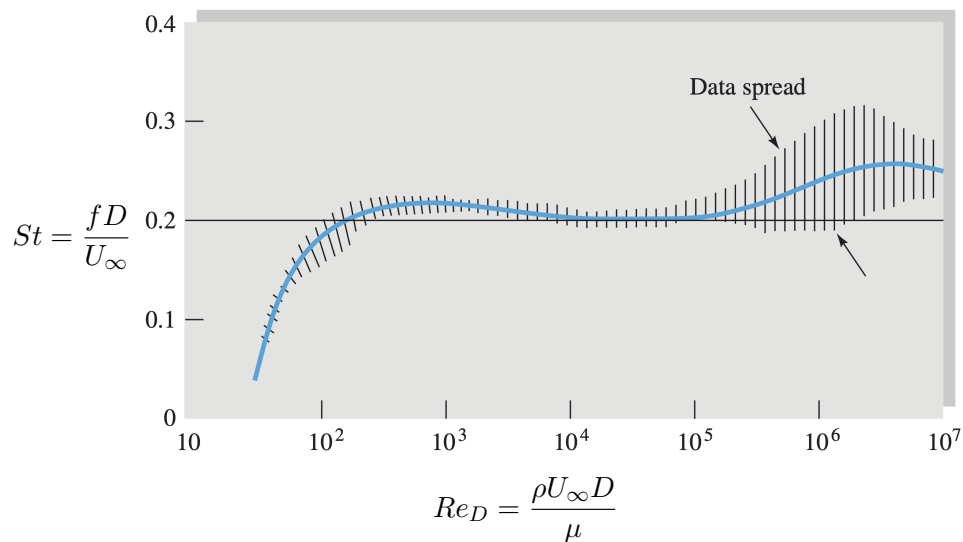
Figure 8.3: Cylinder Strouhal number versus Reynolds number
