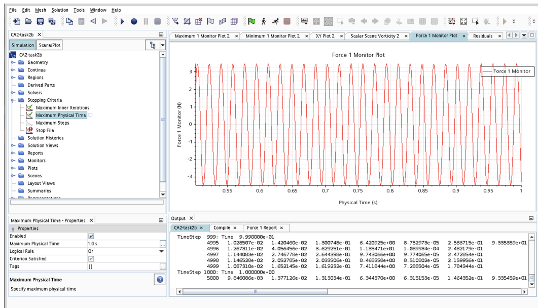
Figure 7.4: Fluctuating cylinder lift force
