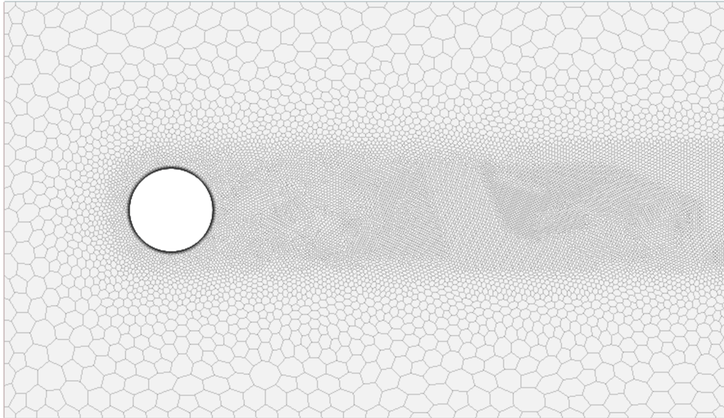
Figure 7.3: Final mesh of the two-dimensional cylinder flow computational domain.
