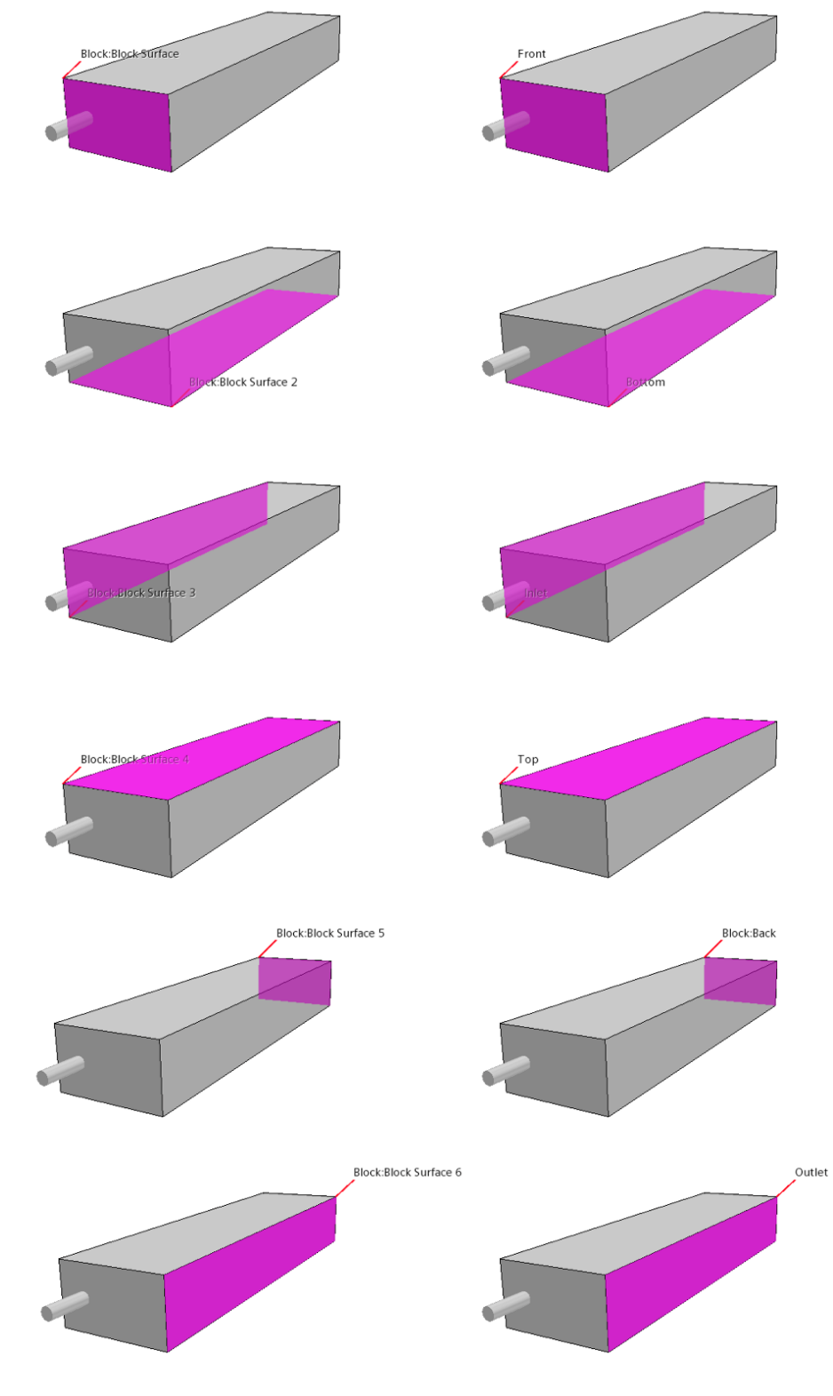
Figure 7.1: Renaming of generated boundary faces
