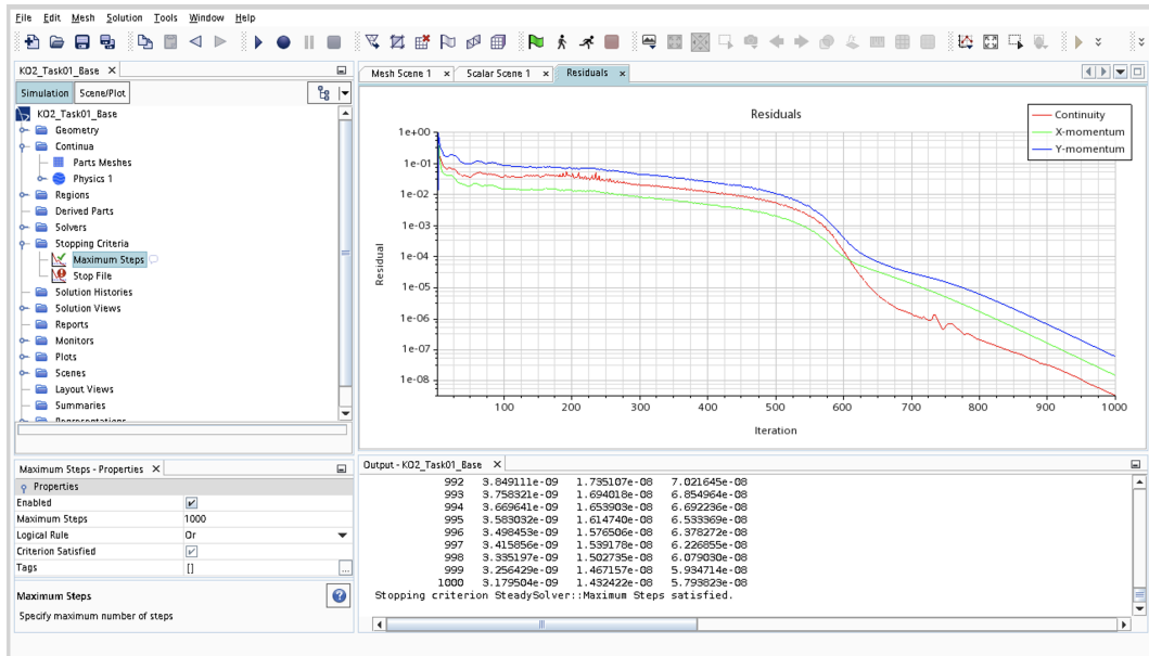
Figure 6.5: Flat-plate boundary layer residual log
