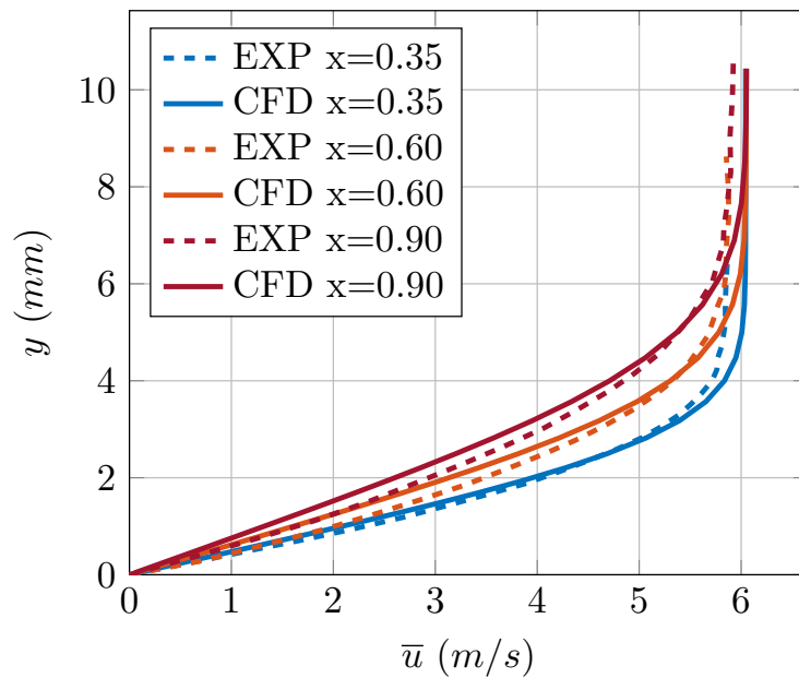
Figure 8.1: Laminar boundary layer velocity profiles – CFD results compared with measured data at three axial positions in a laminar boundary layer.
