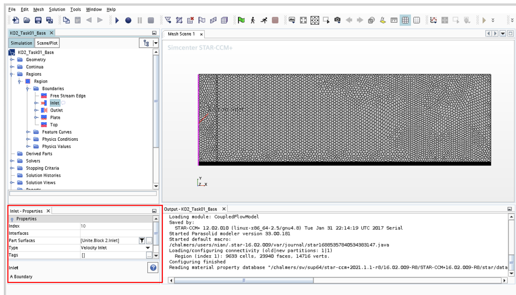
Figure 6.2: Boundary condition properties
