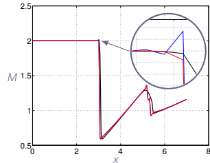
Mach number along line 3
