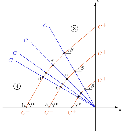
Figure 2: Expansion fan centered at (x, t) = (0.0, 0.0)
