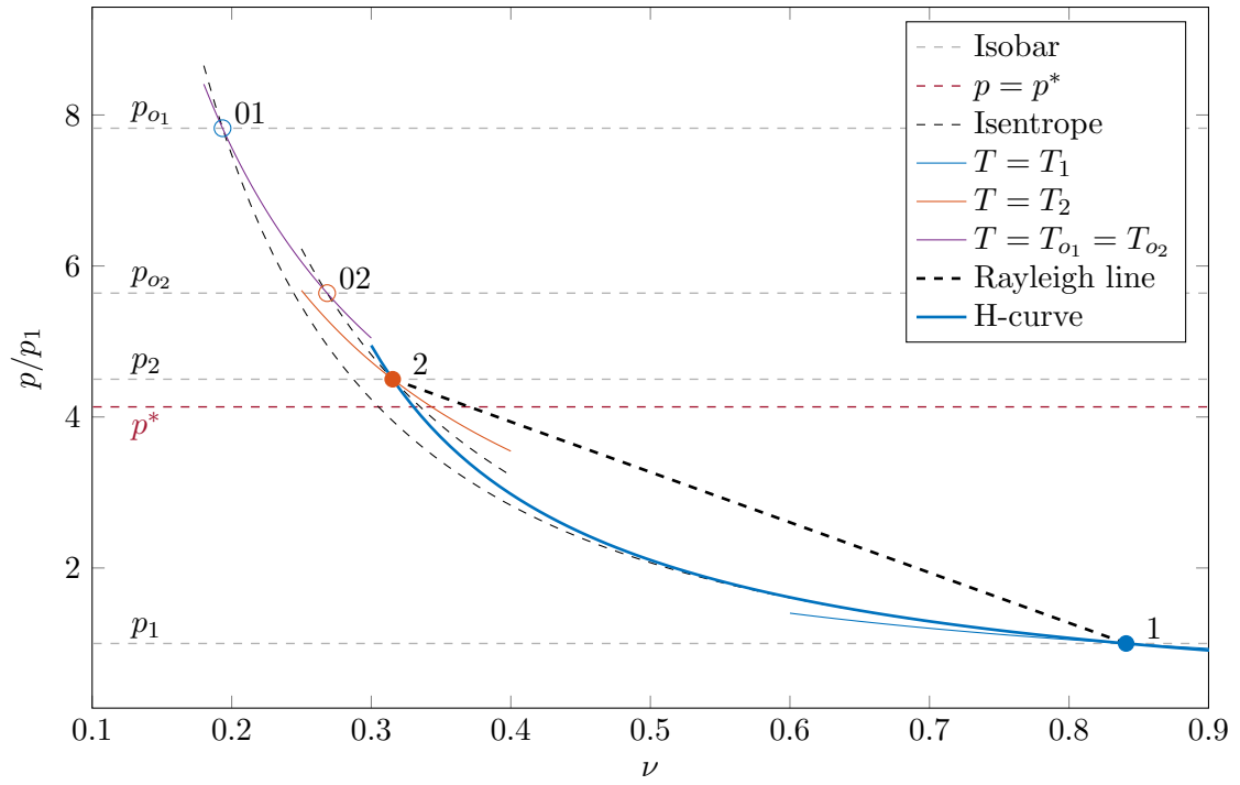
Normal shock ( p\nu -diagram)
